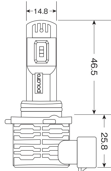
HB3/HB4 TYPE
