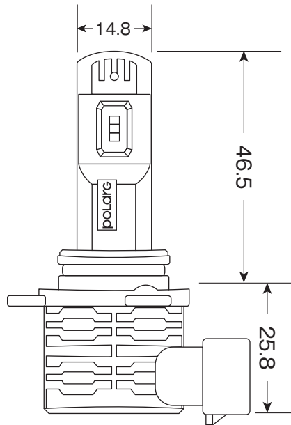
HIR2 TYPE
