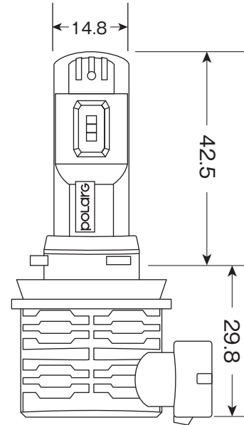
H8/H11/H16 TYPE
